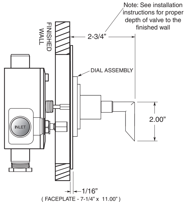
SIDE VIEW - INSTALLED
