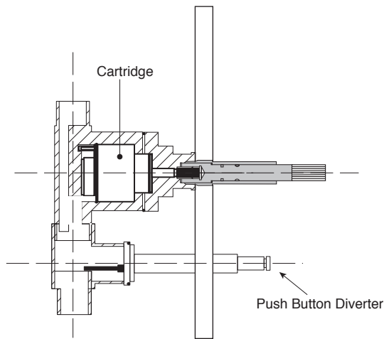
Cutaway View
