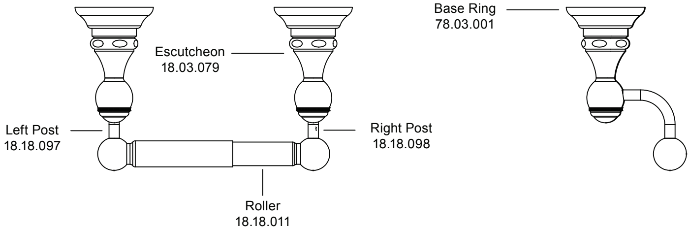
BOTTOM VIEW
