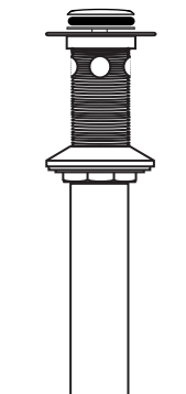
SOFT TOUCH DRAIN ASSEMBLY P/N 18.11.052
